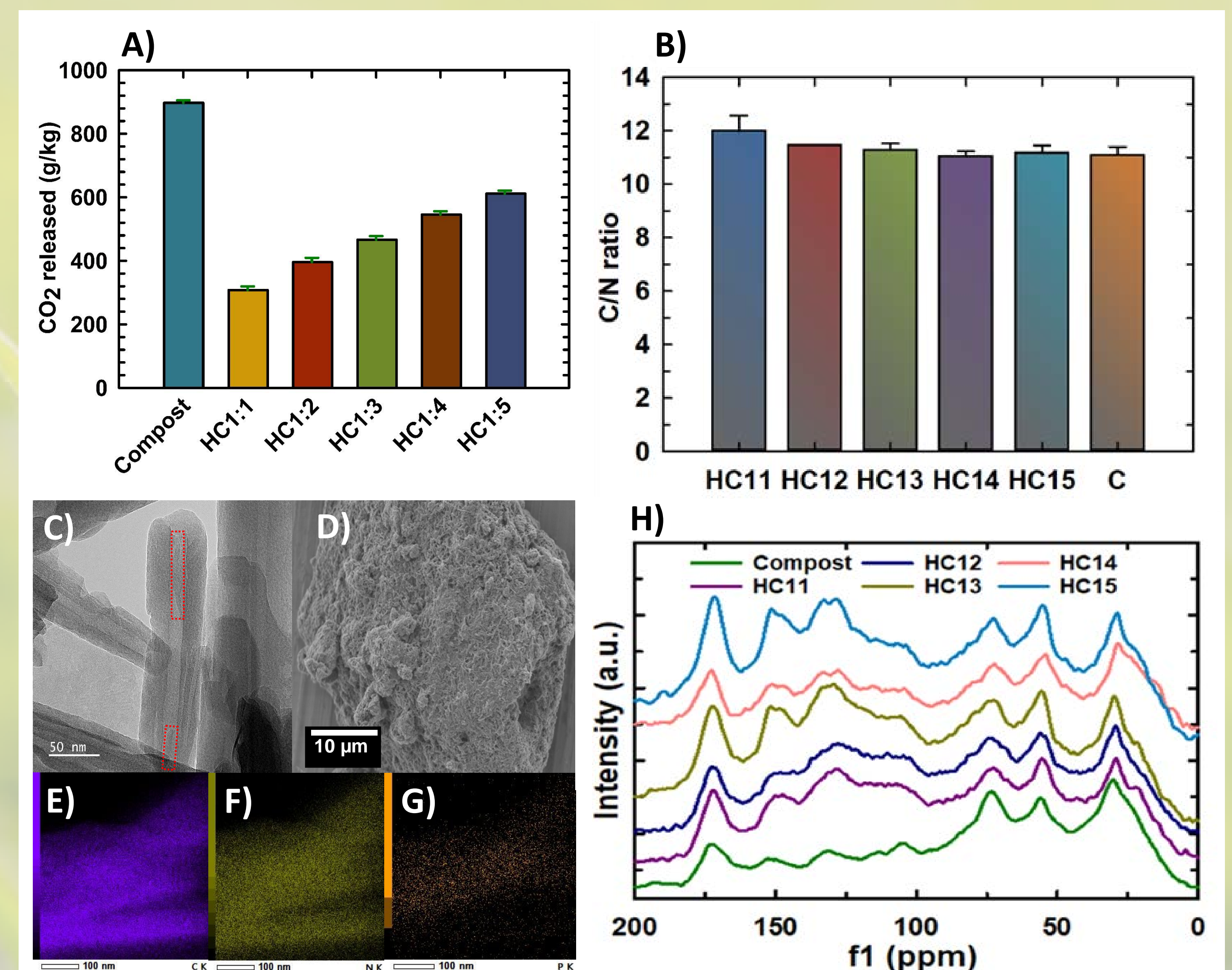
A) Microbial CO 2 respiration analysis; B) C/N Ratio; C & D) TEM & SEM analysis Halloysite/Compost; E to G) Elemental Mapping of C, N, O and P; and H) 13C NMR analysis
